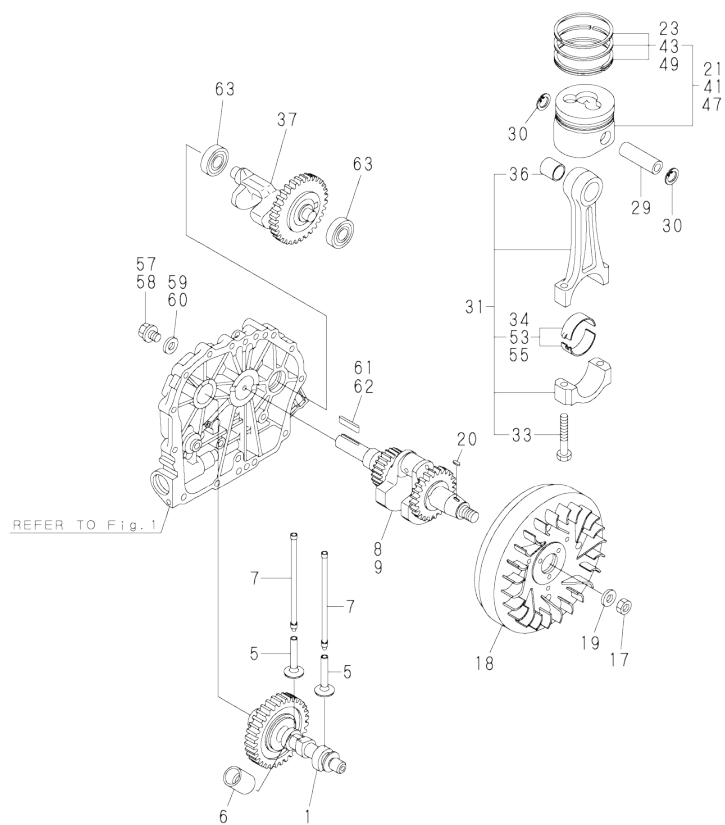
Fig.4. CRANKSHAFT,PISTON & CAMSHAFT
