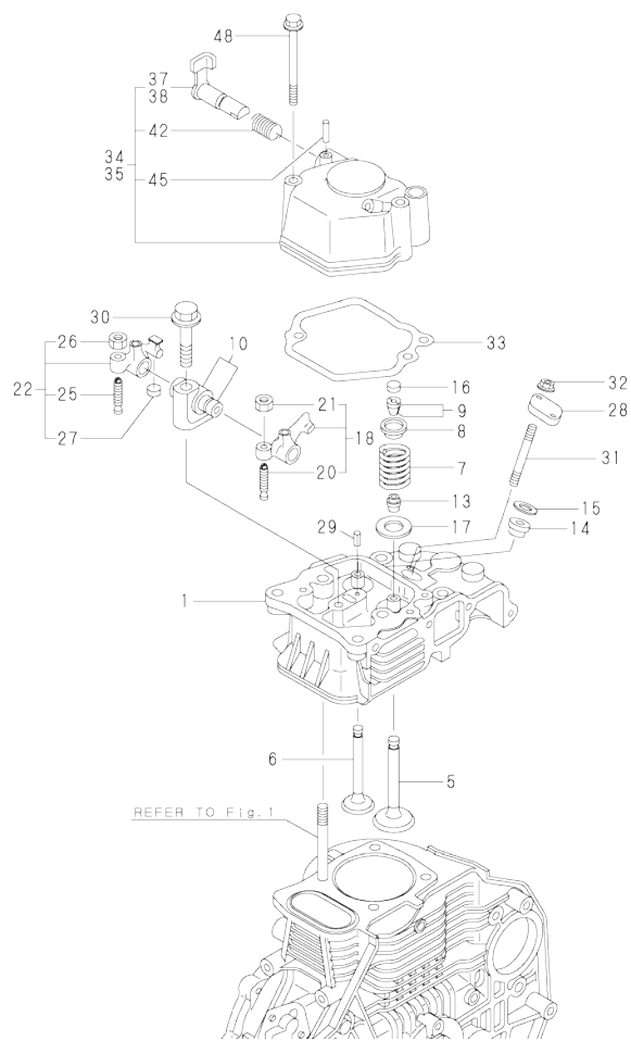
Fig.2. CYLINDER HEAD & BONNET
