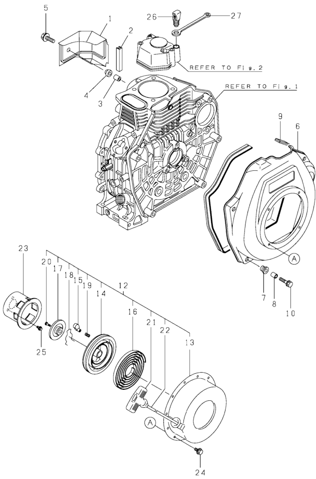
Fig.6. COOLING & STARTING DEVICE
