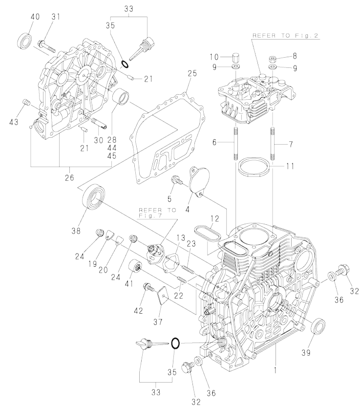
Fig.1. CYLINDER BLOCK
