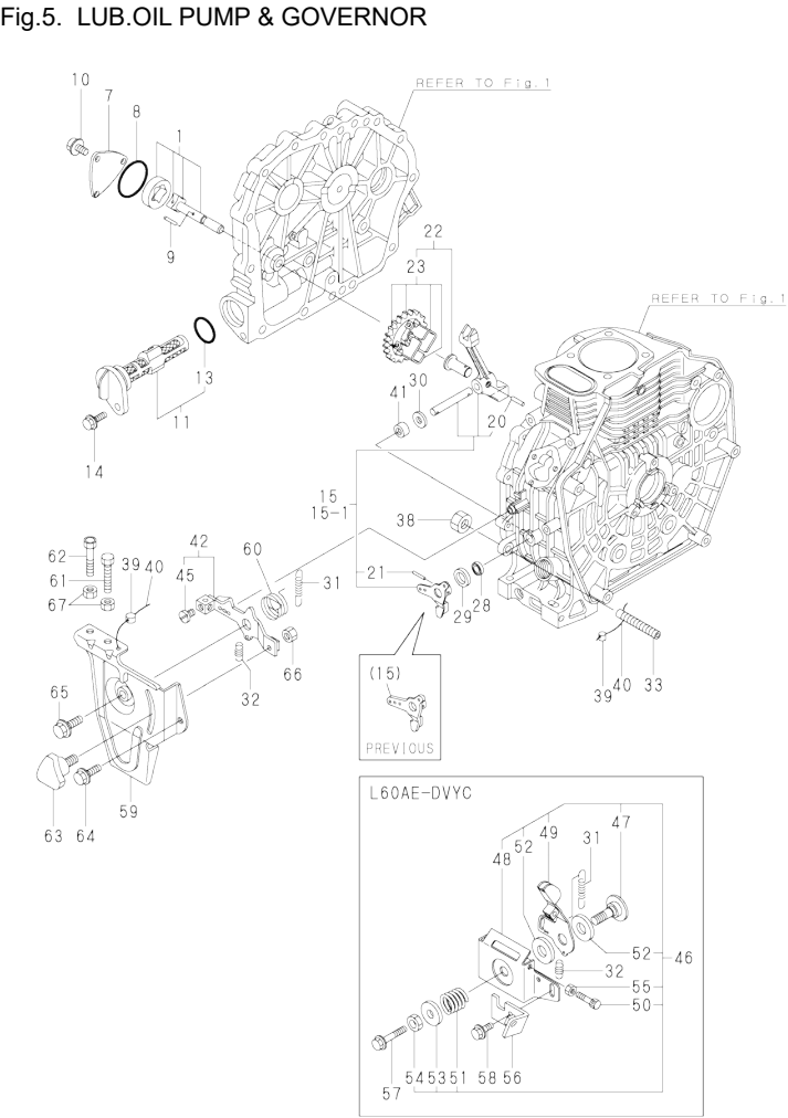
Fig.5. LUB.OIL PUMP & GOVERNOR
