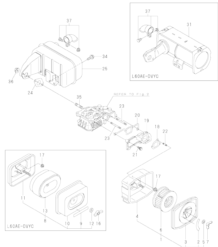
Fig.3. AIR CLEANER & MUFFLER
